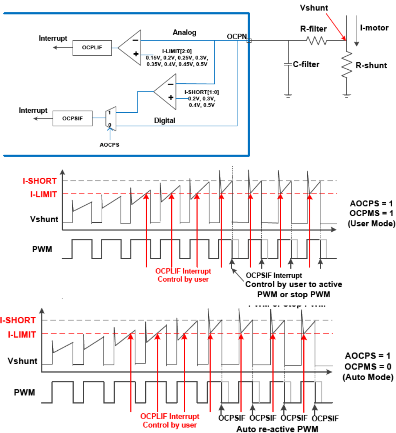
Figure 20.4.2 Analog OCP
