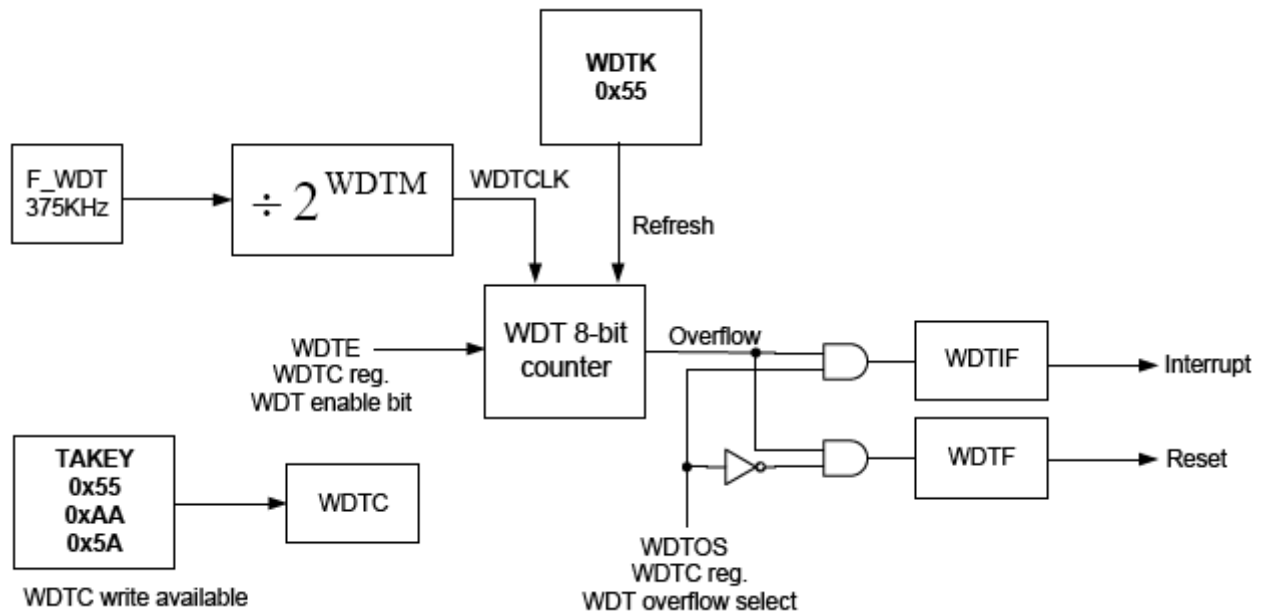
Figure 12.5.1 WDT block diagram
