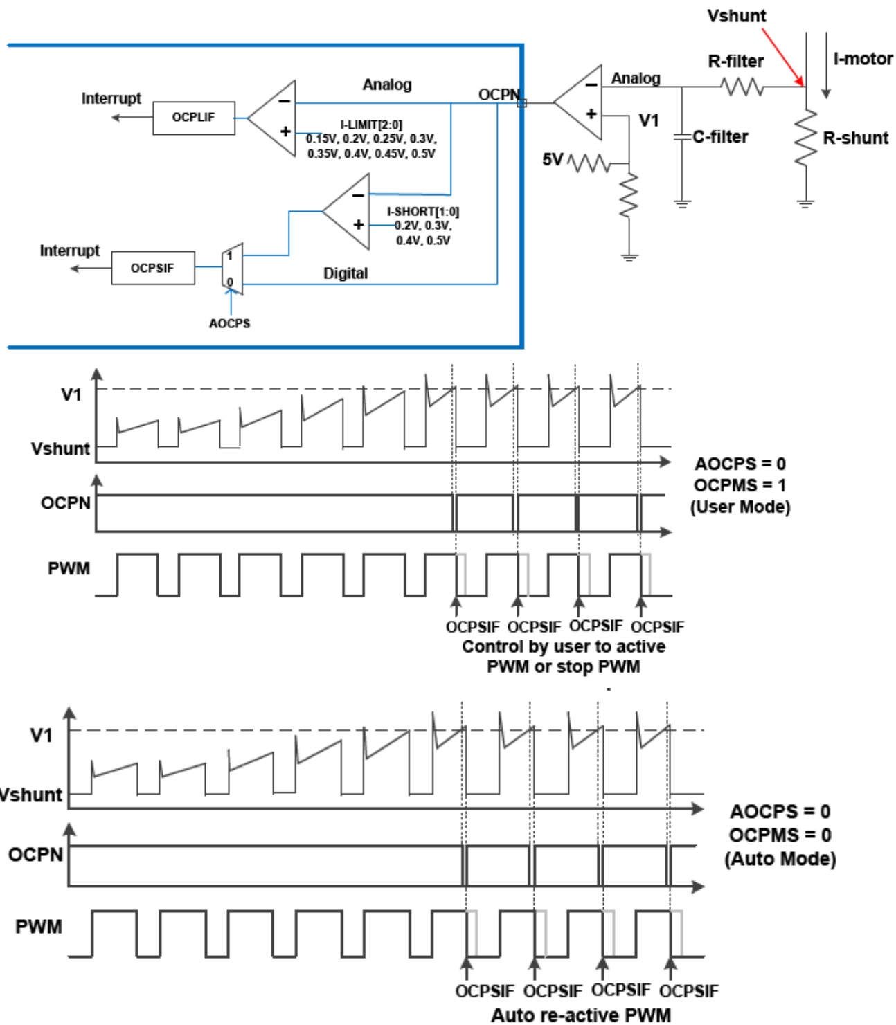
Figure 20.4.1 Digital OCP
