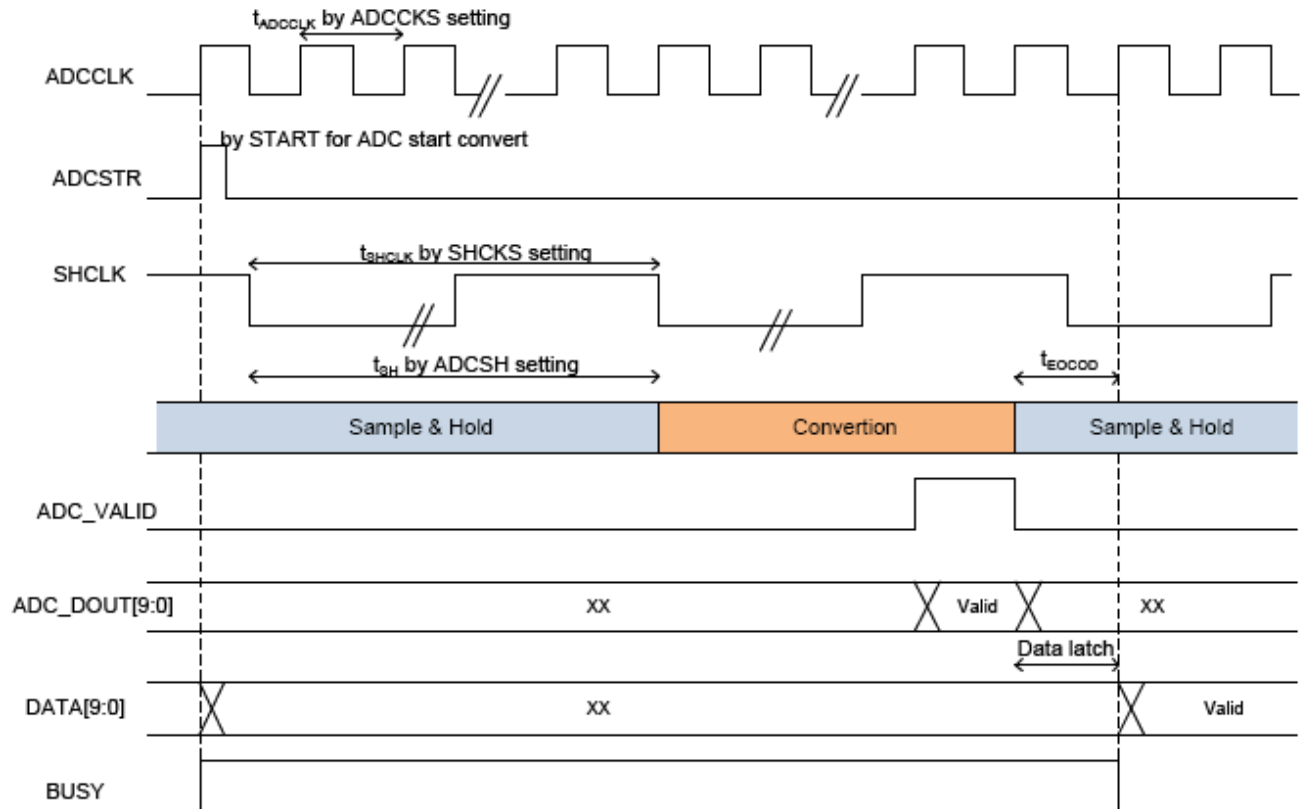
Figure15.1 ADC conversion timing
