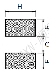
Recommended Land Pattern
