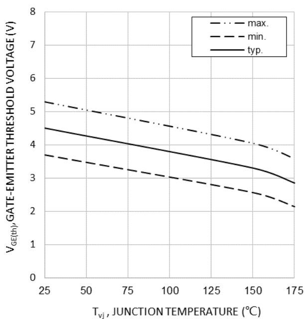
Fig. 5 Gate-emitter threshold voltage as a function of junction temperature ( I_C=0.60mA )
