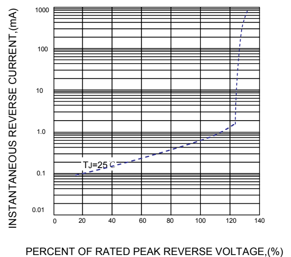
FIG.4-TYPICAL REVER CHARACTERISTICS
