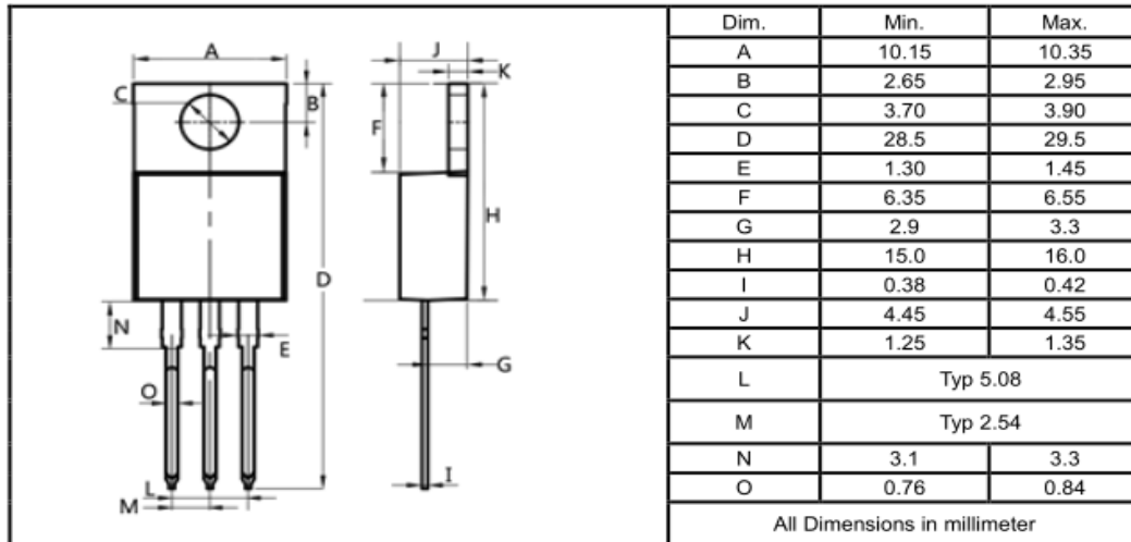
TO-220F
