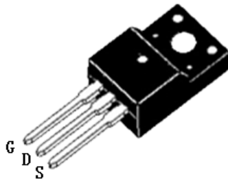
TO-220F
