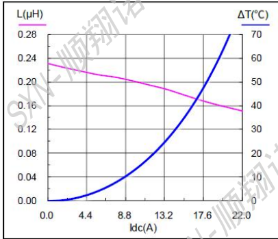
SMMS0530-R68M
