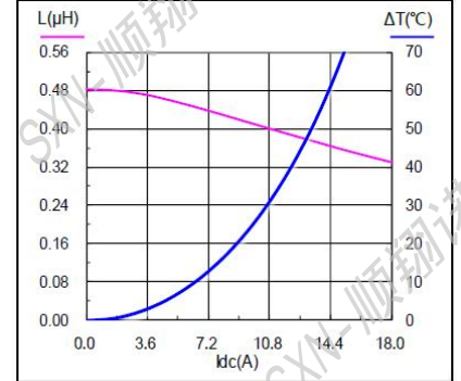
SMMS0530-R47M
