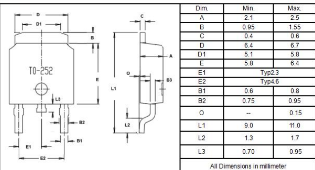
TO-252
