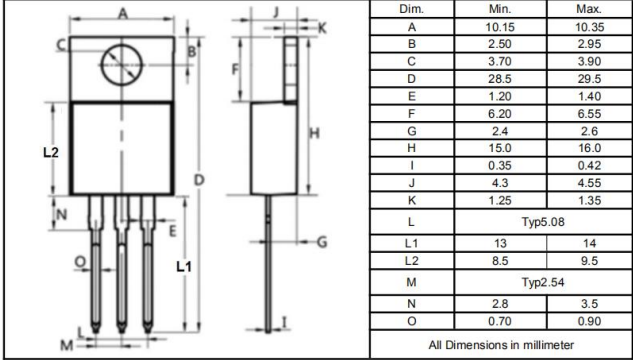
TO-220AB
