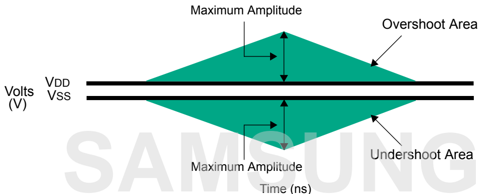
Figure 18. Overshoot and Undershoot Definition
