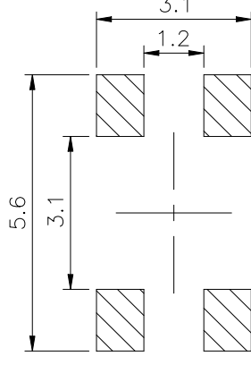
PCB. 焊接图 PCB. WELDING DRAWING
