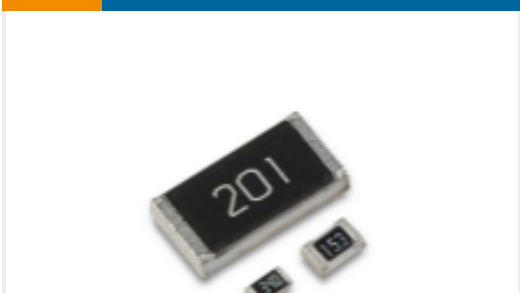
TE Part #1-2176329-3 CRGP 1210 100R 1%
