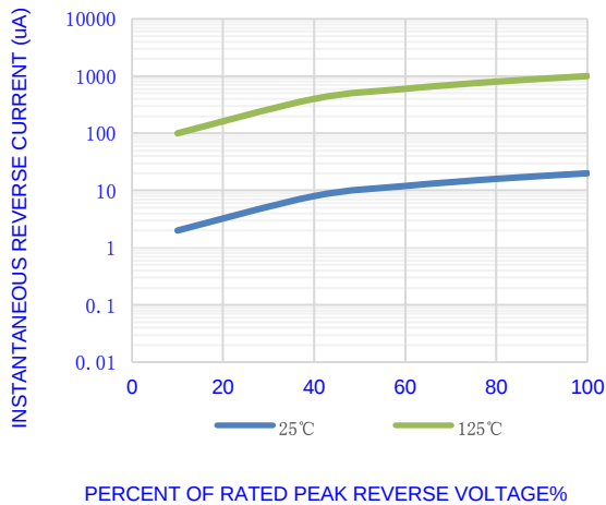
Fig.3-TYPICAL REVERSE CHARACTERISTICS
