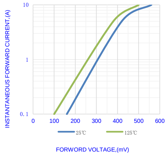
Fig.2-TYPICAL INSTANTANEOUS FORWARD
