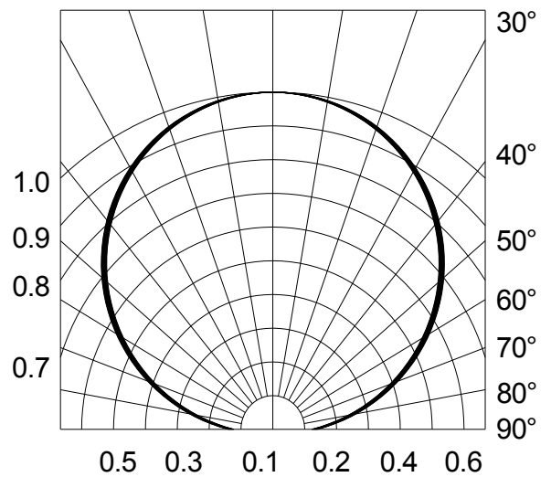
Fig.6-Radiation Diagram Ta=25°C
