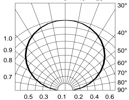
Fig.6-Radiation Diagram
