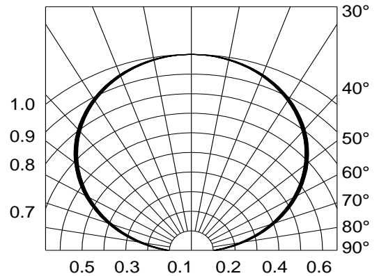
Fig.6-Radiation Diagram Ta=25°C
