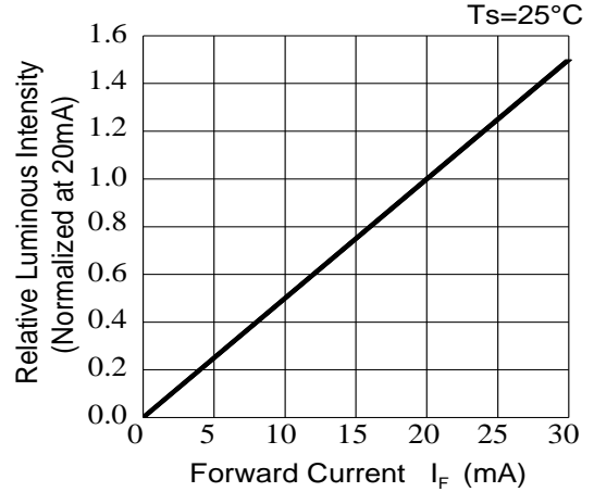
Fig.2-Relative Luminous Intensity vs. Forward Current Ts=25°C
