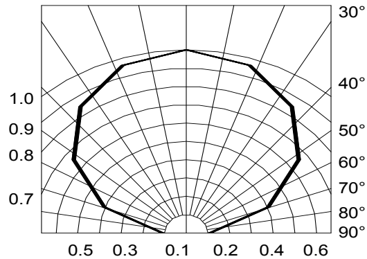
Fig.6-Radiation Diagram Ta=25°C
