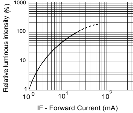
Fig.2 - Relative Luminous Intensity vs. Forward Current Ta=25°C
