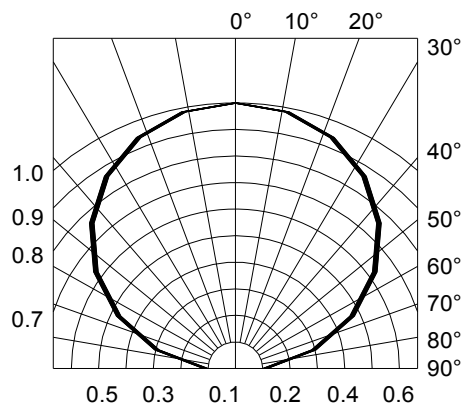
Fig.6-Radiation Diagram Ta=25°C
