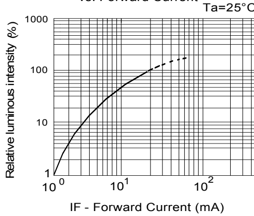
Fig.2 - Relative Luminous Intensity vs. Forward Current Ta=25°C
