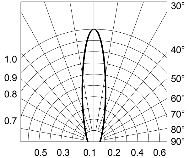
Fig.6-Radiation Diagram T_a=25^\circ\text{C}
