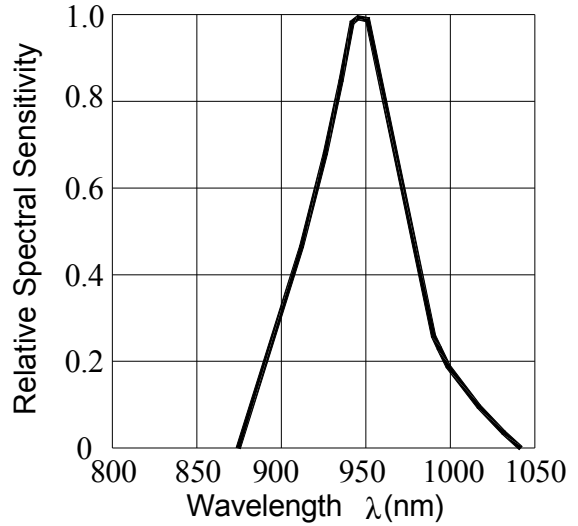
Fig.2-Spectral Sensitivity T_a=25^\circ\text{C}
