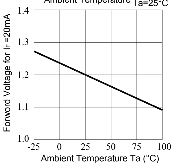
Fig.8-Forward Voltage vs. Ambient Temperature T_a=25^\circ\text{C}
