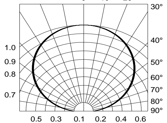
Fig.6-Radiation Diagram
