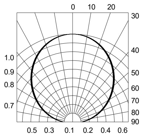
Fig.6-Radiation Diagram
