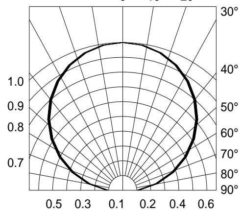
Fig.6-Radiation Diagram Ta=25°C
