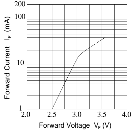
Fig.4-Forward Current vs. Forward Voltage Ta=25°C
