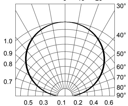
Fig.6-Radiation Diagram
