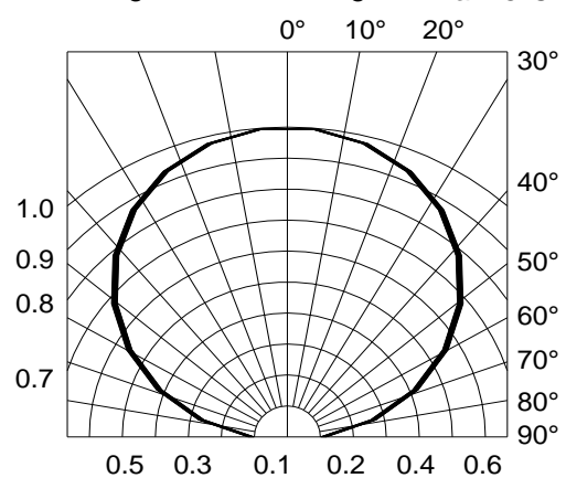
Fig.6-Radiation Diagram
