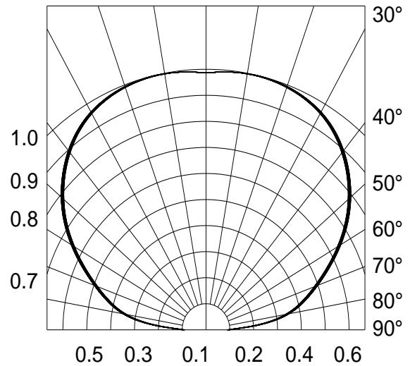
Fig.6-Radiation Diagram Ta=25°C
