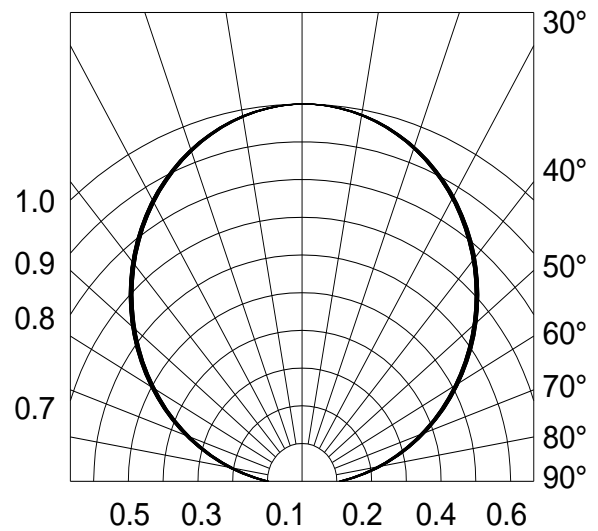
Fig.6-Radiation Diagram T_a=25^\circ\text{C}
