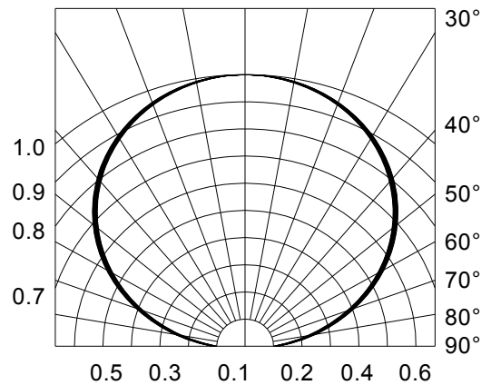
Fig.6-Radiation Diagram Ta=25°C
