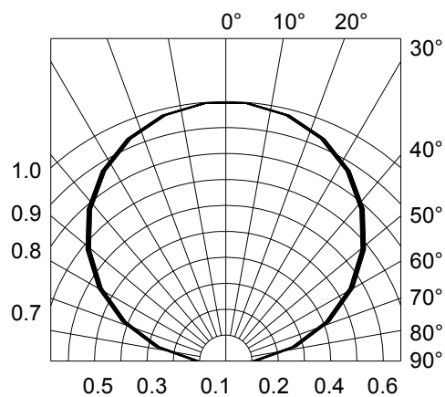
Fig.6-Radiation Diagram Ta=25°C
