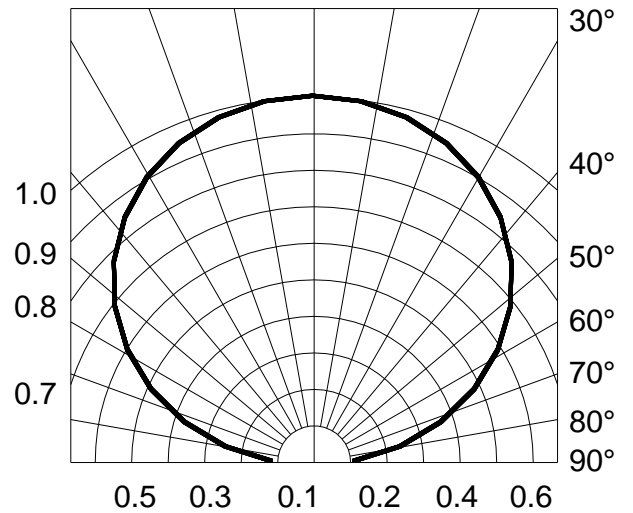
Fig.6-Radiation Diagram Ta=25°C
