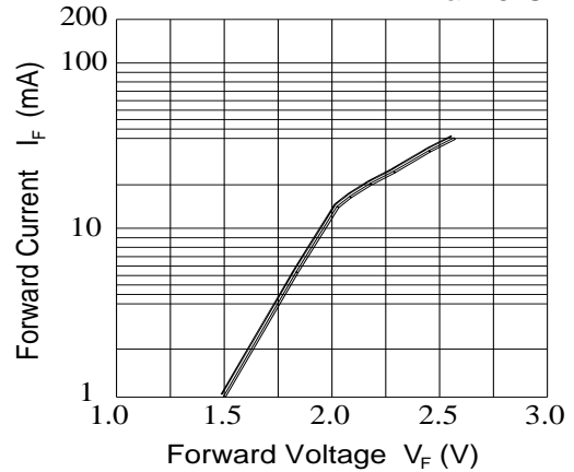
Fig.4-Forward Current vs. Forward Voltage Ta=25°C
