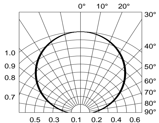
Fig.6-Radiation Diagram
