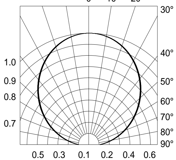
Fig.6-Radiation Diagram Ta=25°C
