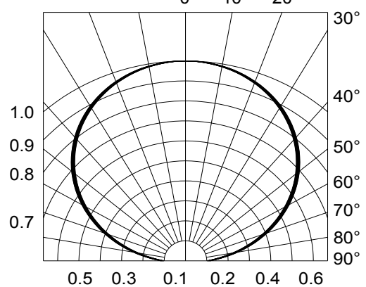
Fig.6-Radiation Diagram T_a=25^\circ\text{C}
