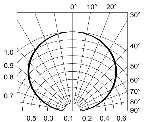
Fig.6-Radiation Diagram Ta=25°C
