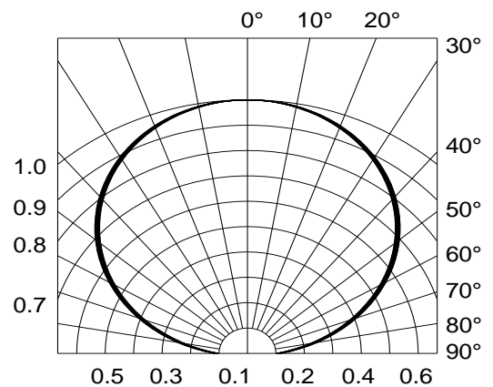
Fig.6-Radiation Diagram
