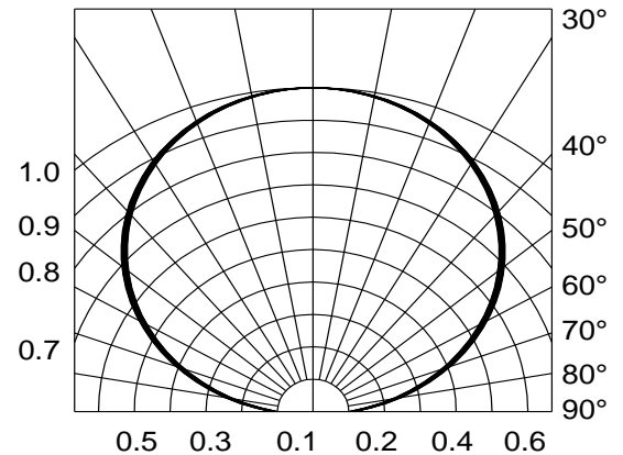
Fig.6-Radiation Diagram Ta=25°C
