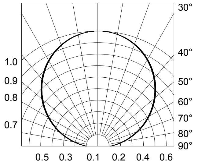
Fig.6-Radiation Diagram Ta=25°C
