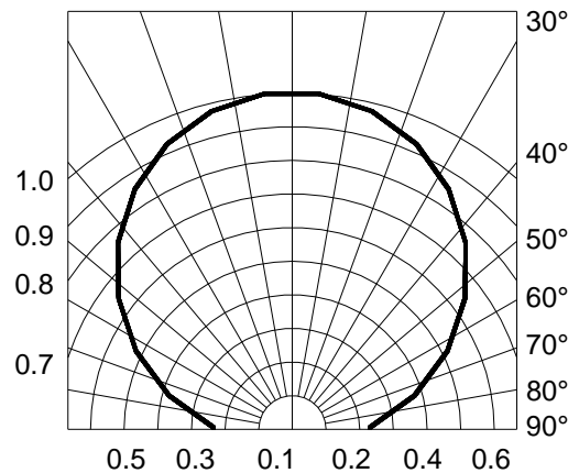
Fig.6-Radiation Diagram Ta=25°C
