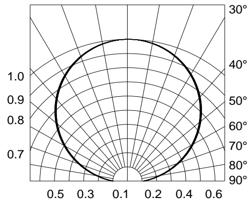
Fig.6-Radiation Diagram
