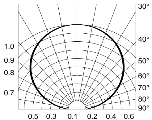
Fig.6-Radiation Diagram
