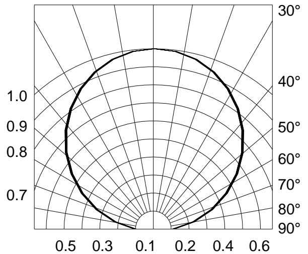
Fig.6-Radiation Diagram Ta=25°C 0° 10° 20°
