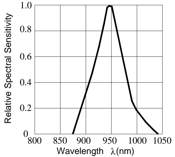
Fig.2-Spectral Sensitivity Ta=25°C
