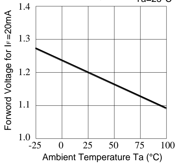
Fig.8-Forward Voltage vs. Ambient Temperature Ta=25°C
