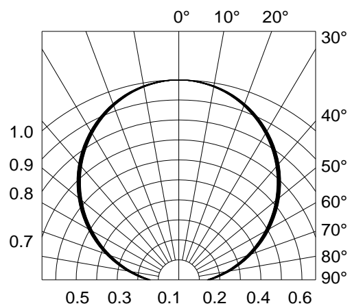
Fig.6-Radiation Diagram Ta=25°C
