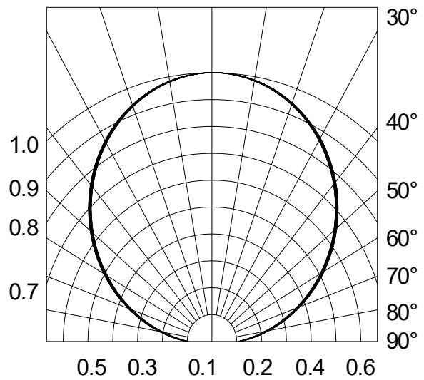
Fig.6-Radiation Diagram Ta=25°C
