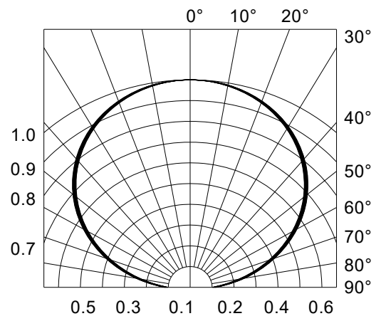
Fig.6-Radiation Diagram
