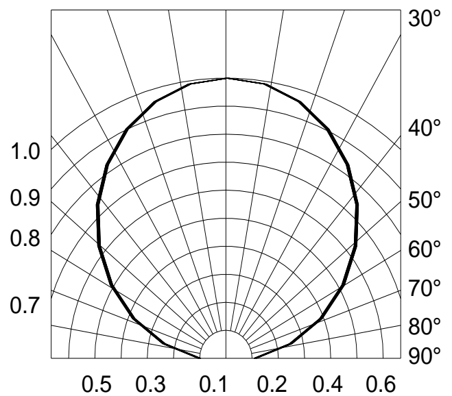
Fig.6-Radiation Diagram Ta=25°C
