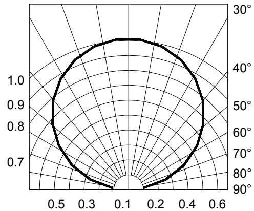
Fig.6-Radiation Diagram
