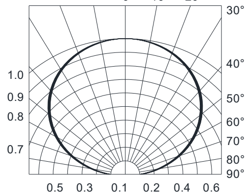
Fig.6-Radiation Diagram
