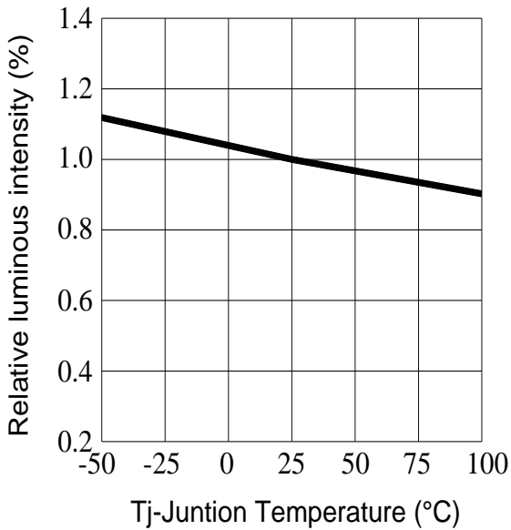
Fig.3-Relative Luminous Intensity vs.Junition Temperature
