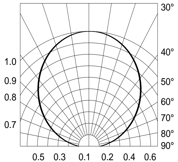
Fig.6-Radiation Diagram T_a=25^{\circ}\text{C}
