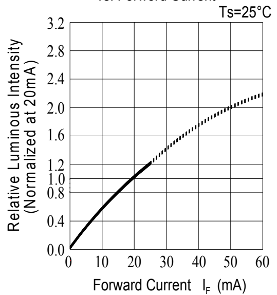
Fig.2-Relative Luminous Intensity vs. Forward Current T s =25°C
