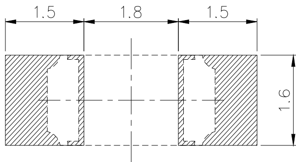
Recommended Solder Pad
