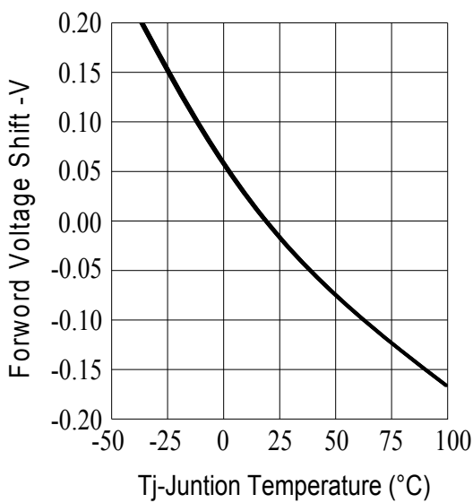
Fig.1-Forward Voltage Shift vs. Junction Temperature
