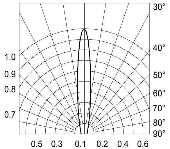
Fig.6-Radiation Diagram Ta=25°C
