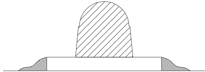
Recommended Solder Pad
