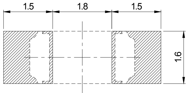
Recommended Solder Pad
