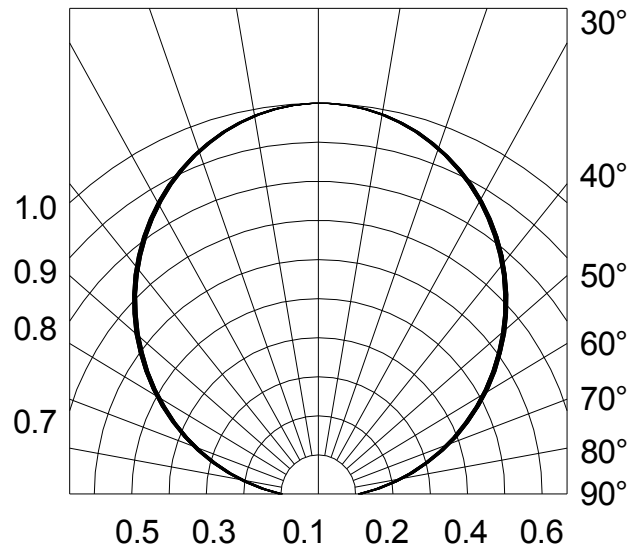
Fig.6-Radiation Diagram Ta=25°C
