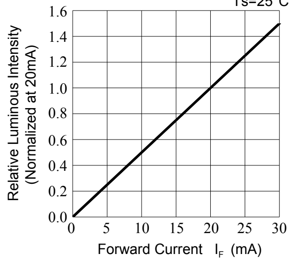
Fig.2-Relative Luminous Intensity vs. Forward Current T s =25°C
