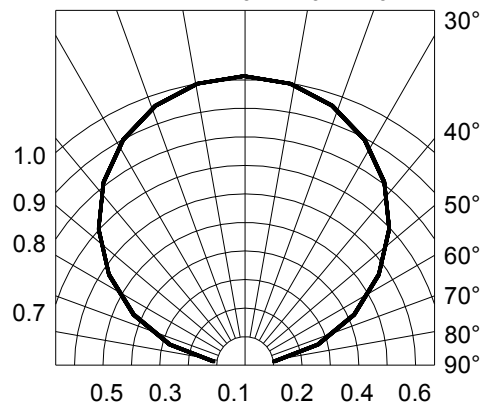
Fig.6-Radiation Diagram Ta=25°C
