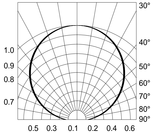
Fig.6-Radiation Diagram Ta=25°C
